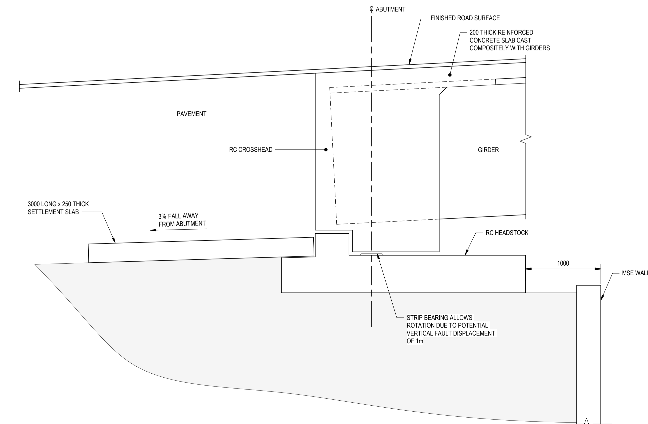
B SECTION S101 SCALE 1:25
