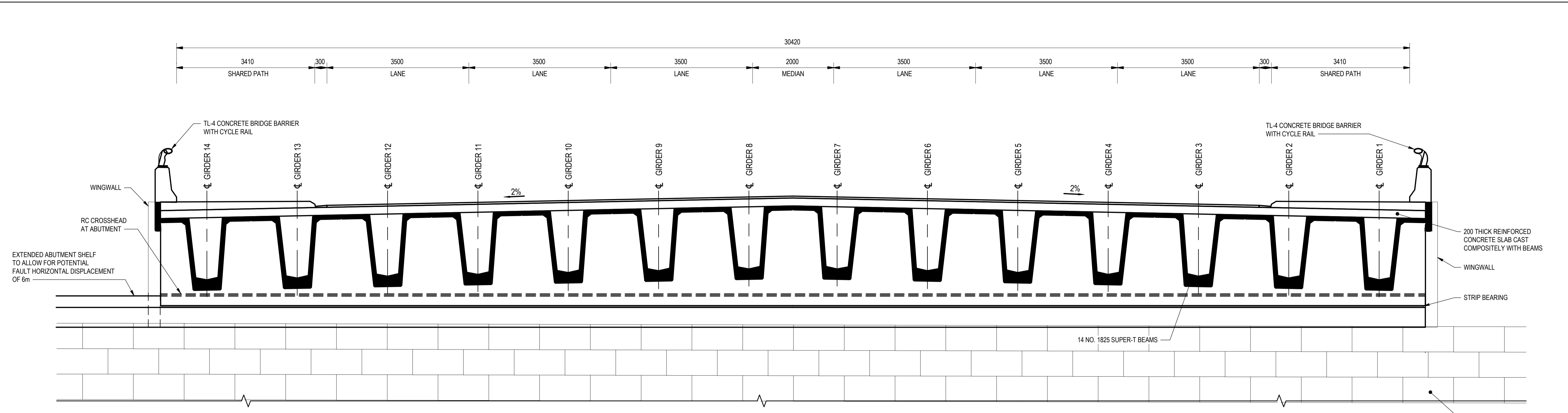
A SECTION S101 SCALE 1:50
